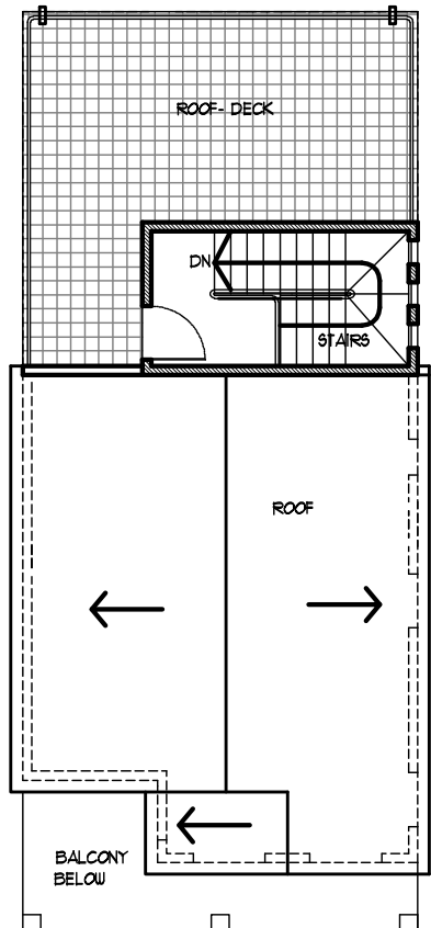
ROOF DECK PLAN
